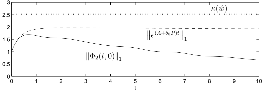
Figure 2: Norms of the evolution operator/matrix exponential and upper bound \kappa(\hat{w})
