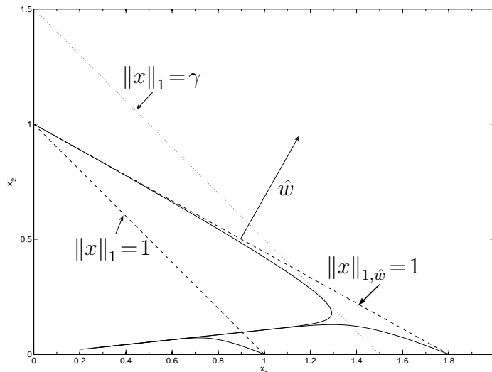
Figure 1: Linear Lyapunov function
