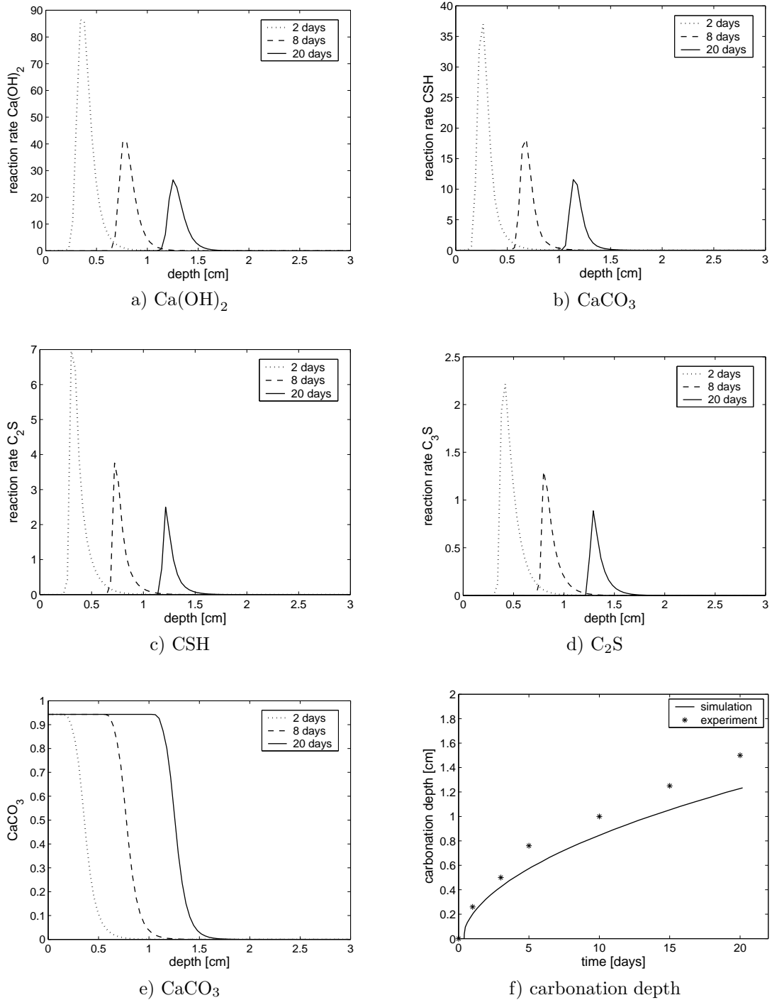
Figure 7: Production rates, profile of CaCO 3 as well as carbonation depth obtained with carbonation-reaction rates ten times faster than in the standard setting.
