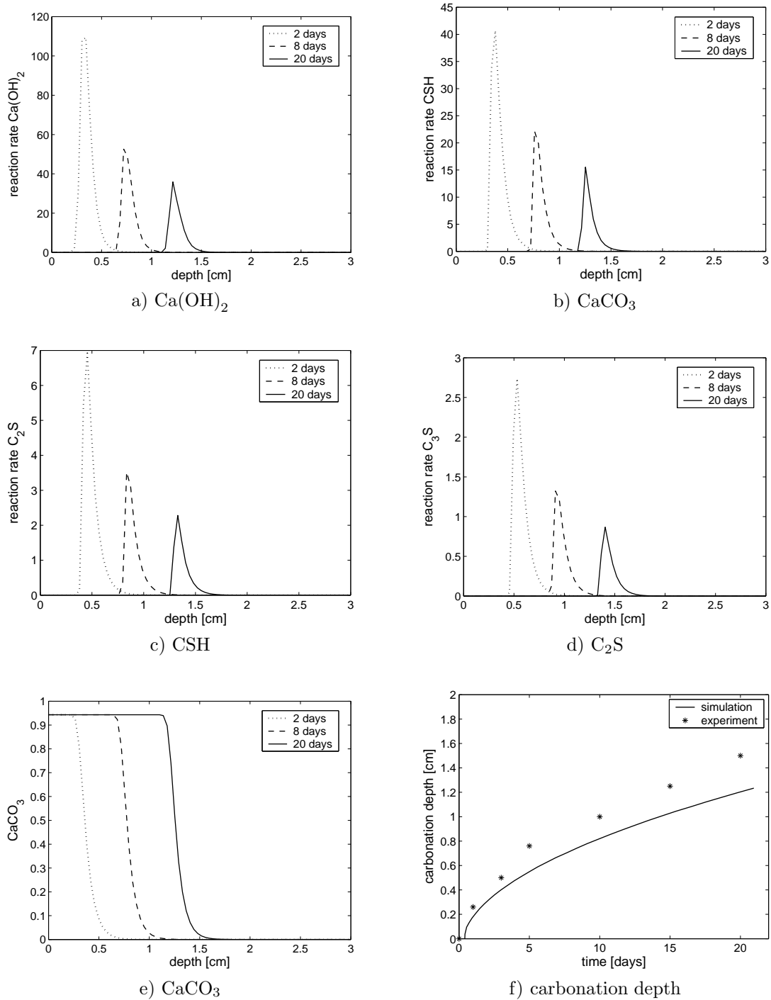
Figure 8: Production rates, profile of CaCO 3 as well as carbonation depth obtained with carbonation-reaction rates one hundred times faster than in the standard setting.
